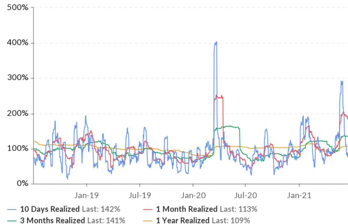
ETHUSD Realized Volatility
