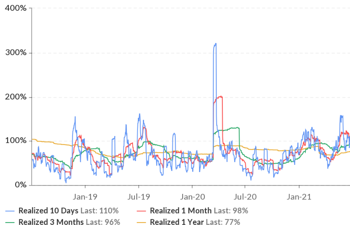
BTCUSD Realized Volatility
